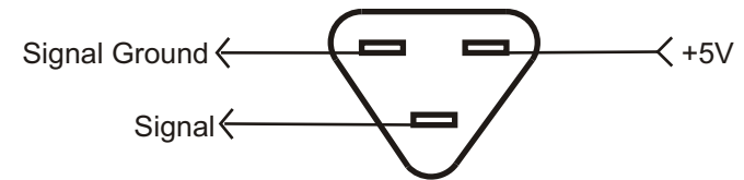
Looking into MAP Sensor Connector (Male Terminals)
