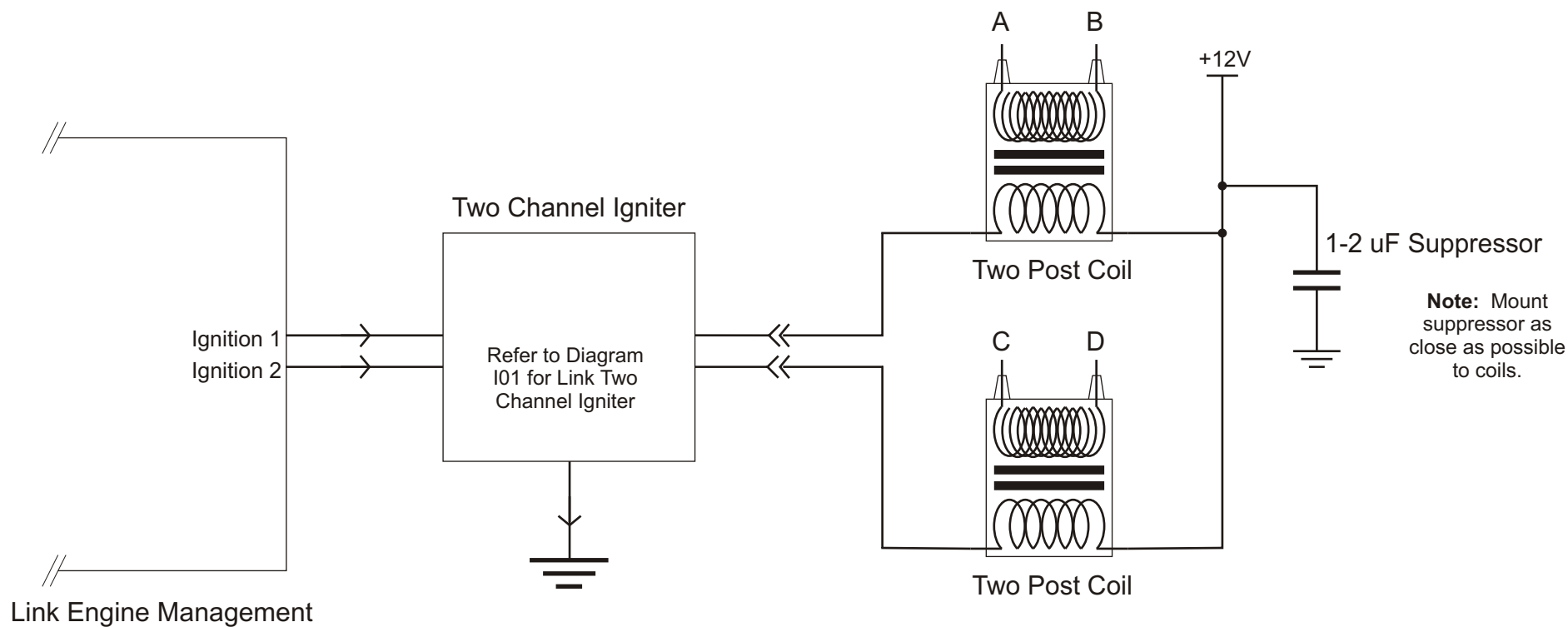
Figure I04.1 - Four Cylinder Wasted Spark Ignition Wiring
