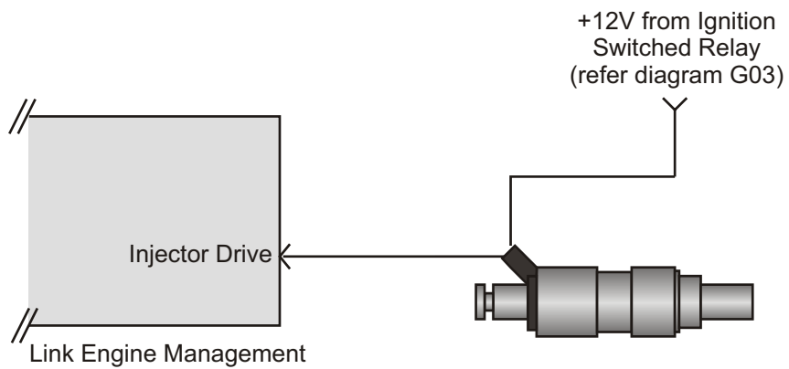
Figure G05.1 - Injector Wiring (High Impedance Injector or Peak and Hold)
