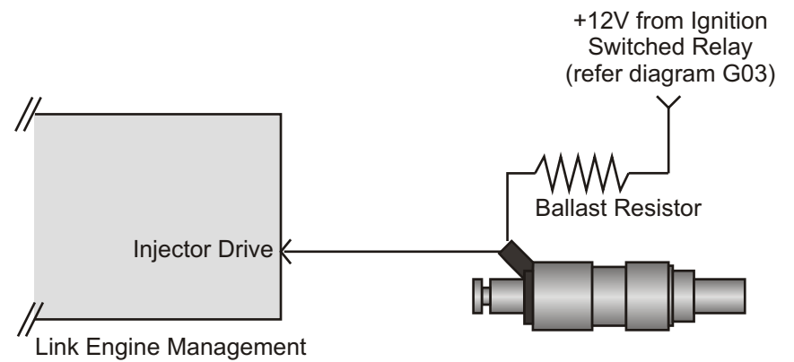
Figure G06.1 - Injector Wiring (Low Impedance Injector)
