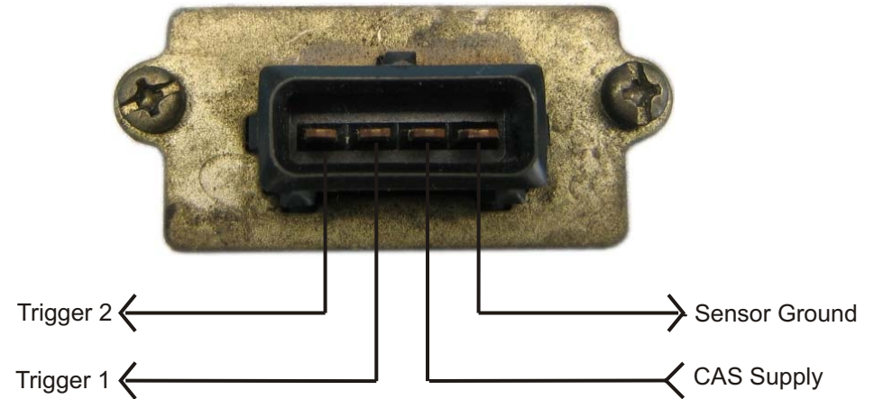
Figure C09.3 - Nissan VH 45 Crank Angle Sensor Wiring (G3 ECU's)
