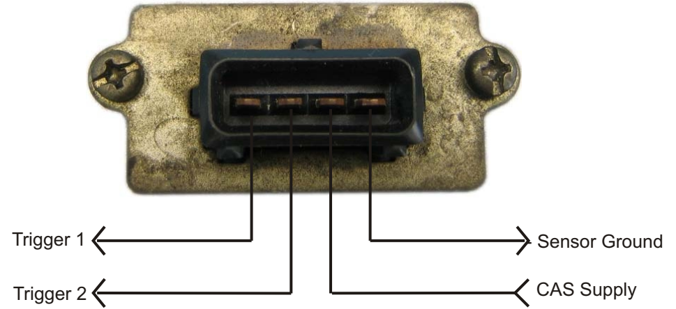
Figure C09.2 - Nissan VH 45 Crank Angle Sensor Wiring (non G3 ECU's)
