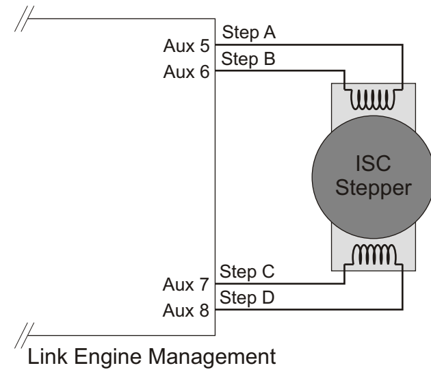
Figure A02.4 - Four Terminal ISC Stepper Wiring
