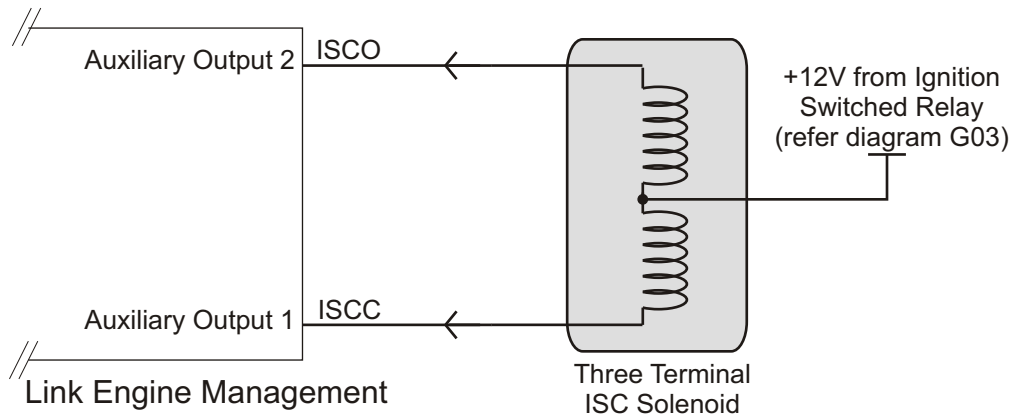
Figure A02.3 - Three Terminal ISC Solenoid Wiring
