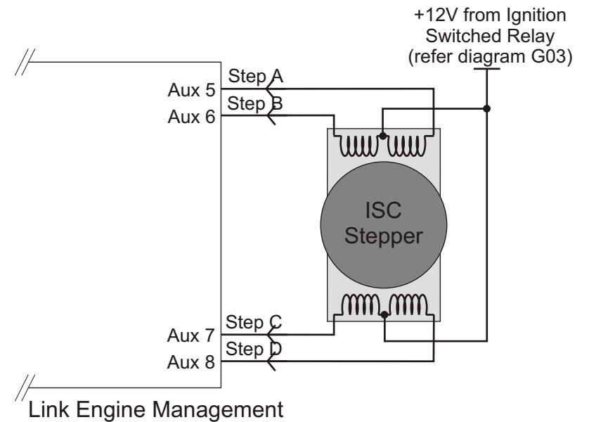
Figure A02.5 - Six Terminal ISC Stepper Wiring
