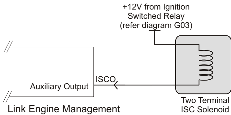
Figure A02.1 - Two Terminal ISC Solenoid Wiring
