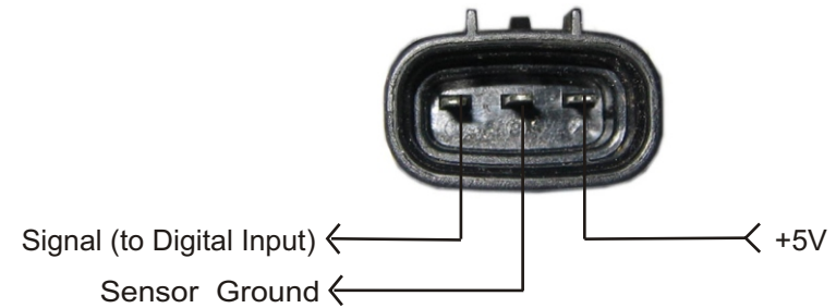
Figure S08.2 - Toyota Speed Sensor Pinout
