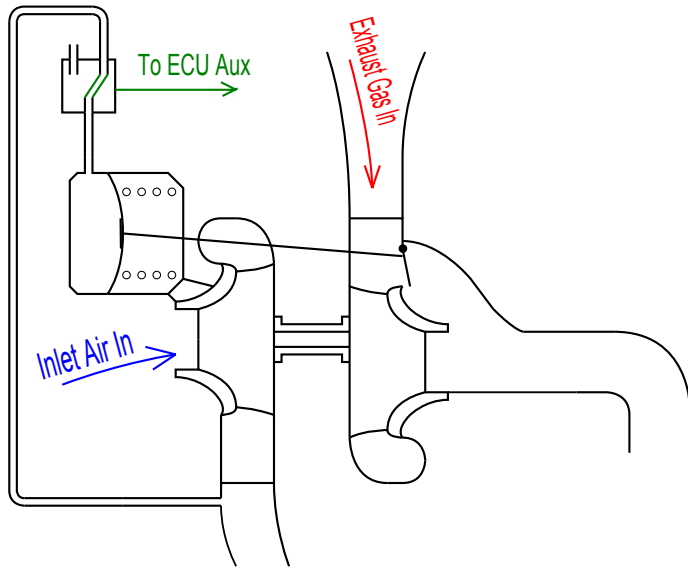
3 Port Internal Wastegate
