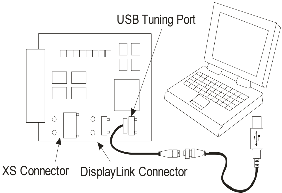
Figure 3.1 – WRXLink G3 Tuning Cable Connection
