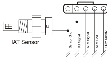
Figure S05.1 - WRX V7-9 IAT to AFM Wiring
