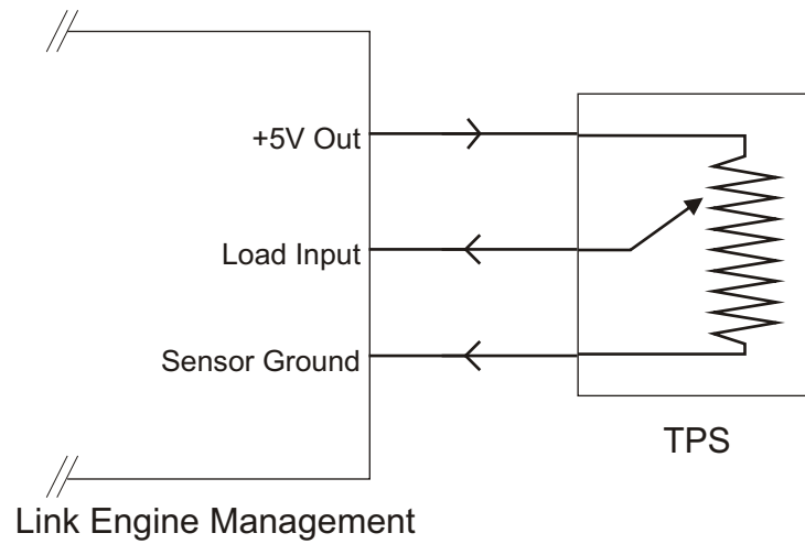
Figure S06.1 - Generic TPS Sensor Wiring
