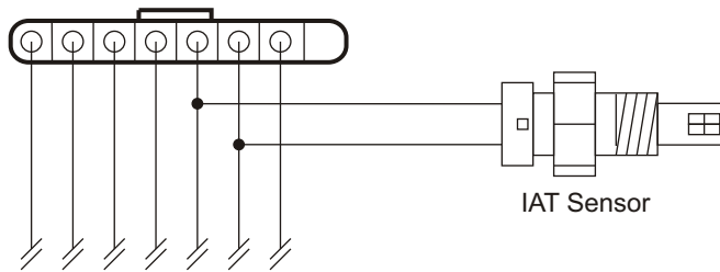
Figure S04.1 - EVO 1-3 IAT to AFM Wiring
