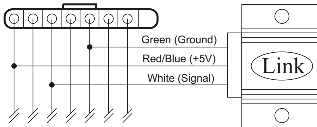
Figure S03.1 - EVO 1-3 MAP to AFM Wiring
