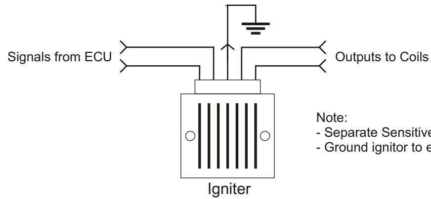
Figure I10.2 - Separation of Ignitor Wiring
