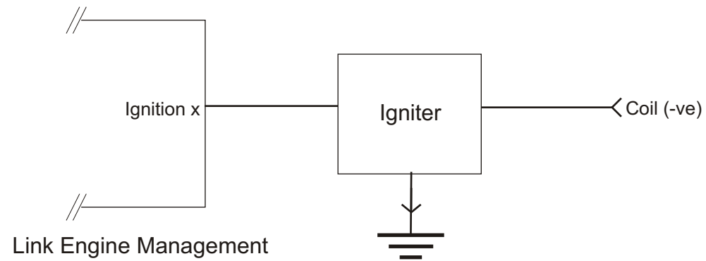
Figure I10.1 - General Ignitor Wiring
