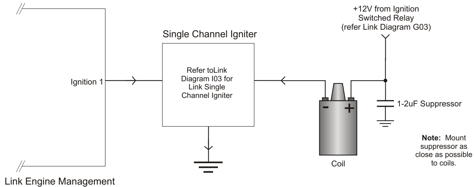
Figure I09.1 - Four Cylinder Wasted Spark Ignition Wiring
