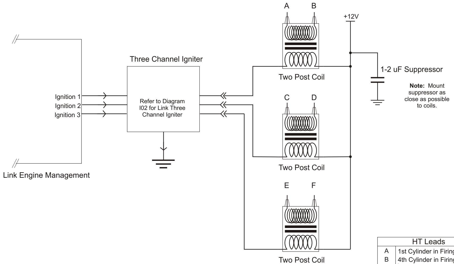
Figure I05.1 - Six Cylinder Wasted Spark Ignition Wiring
