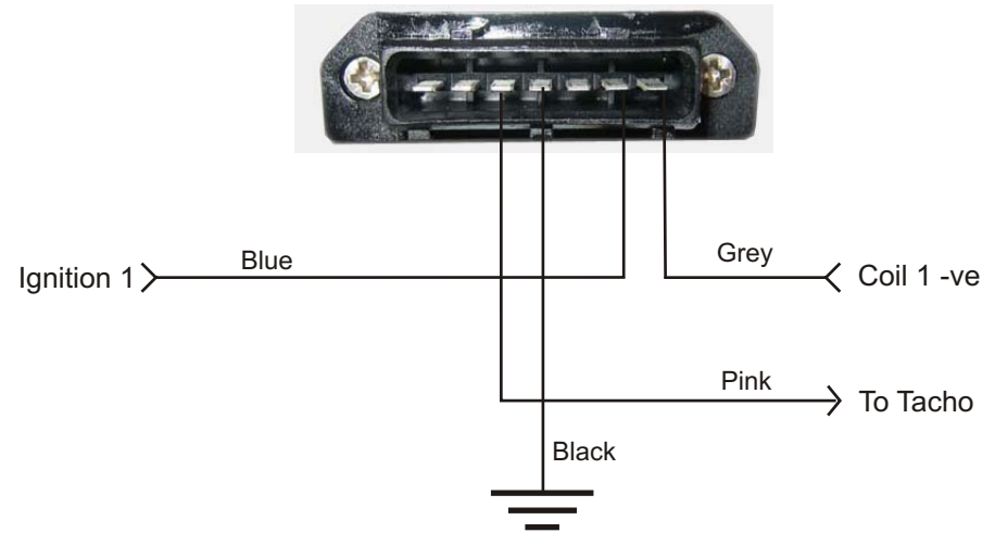
Figure I03.2 - Link Single Channel Igniter Pinout
