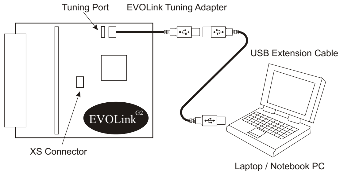
Figure G01.1 - EVOLink Tuning Cable Connection
