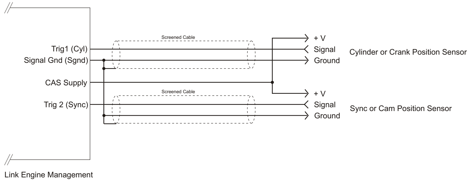
Figure C03.1 - Link Opto/Hall Trigger Wiring
