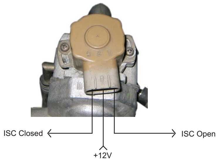
Figure A01.1 - Subaru Idle Control Valve Wiring
