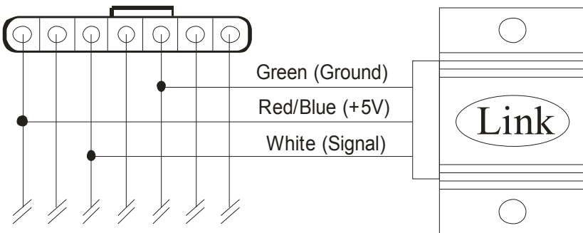
Looking into back (wire side) of the Air Flow Meter Connector
