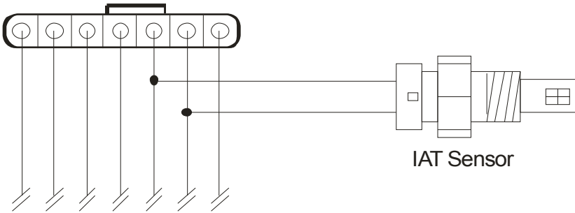
Looking into back (wire side) of the Air Flow Meter Connector
